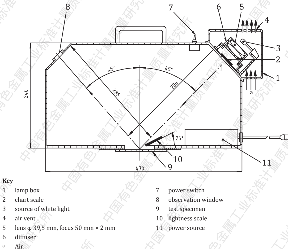
Figure 2 — Diagram of a typical observation box
